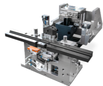
STRIPPING THE INNER CONDUCTOR
